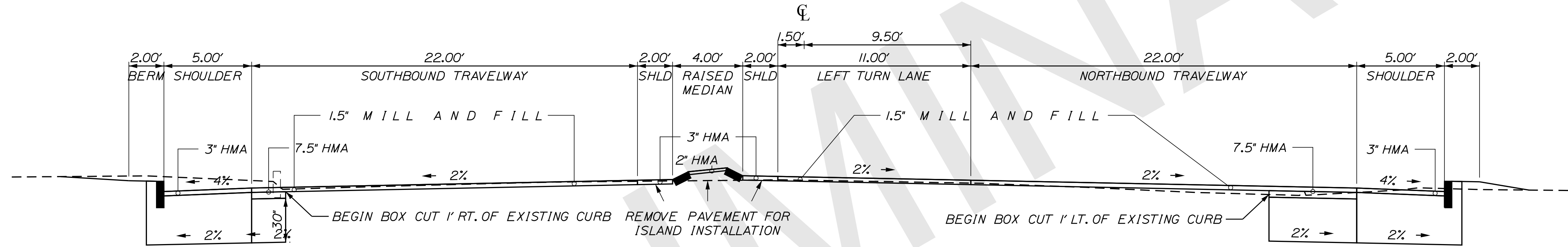
NORMAL NORTHBOUND LEFT TURN LANE
