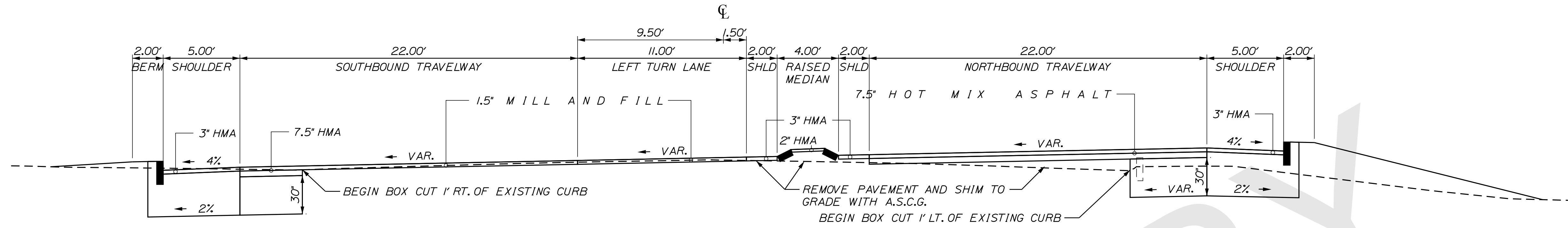
SUPERELEVATED SOUTHBOUND LEFT TURN LANE
